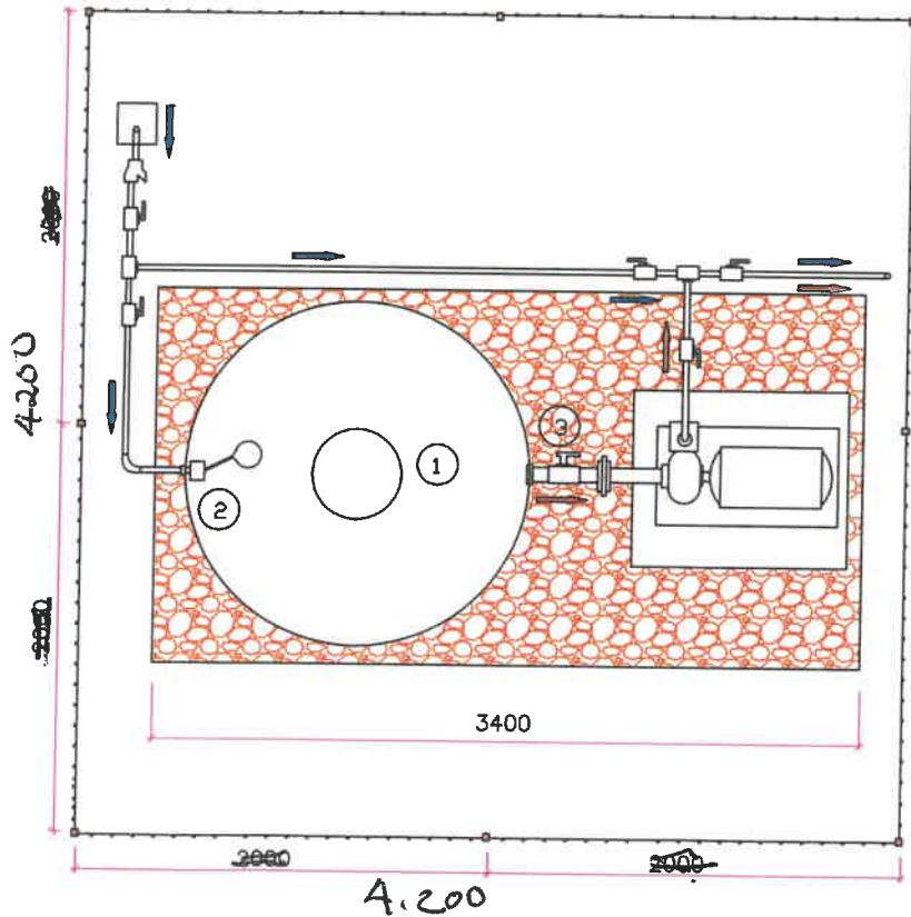
JO JO TANK INSTALLATIONS DETAILS
