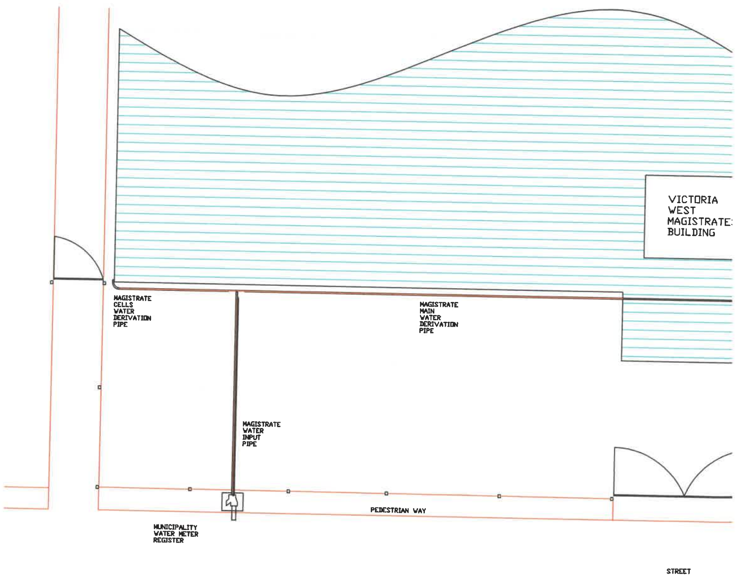
VICTORIA WEST MAGISTRATES J0-J0 TANK INSTALLATION
