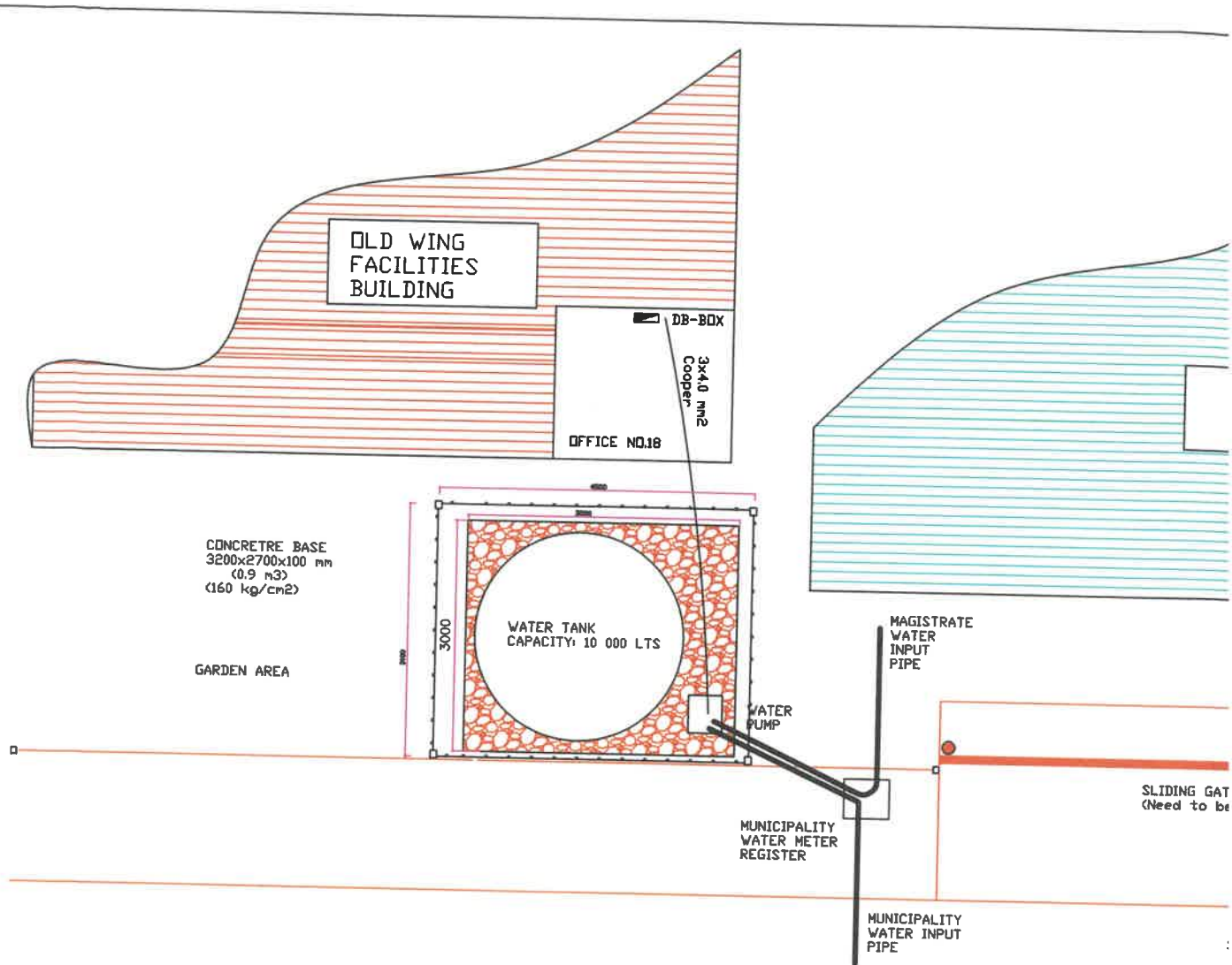
DE AAR MAGISTRATES JO-JO TANK INSTALLATION
