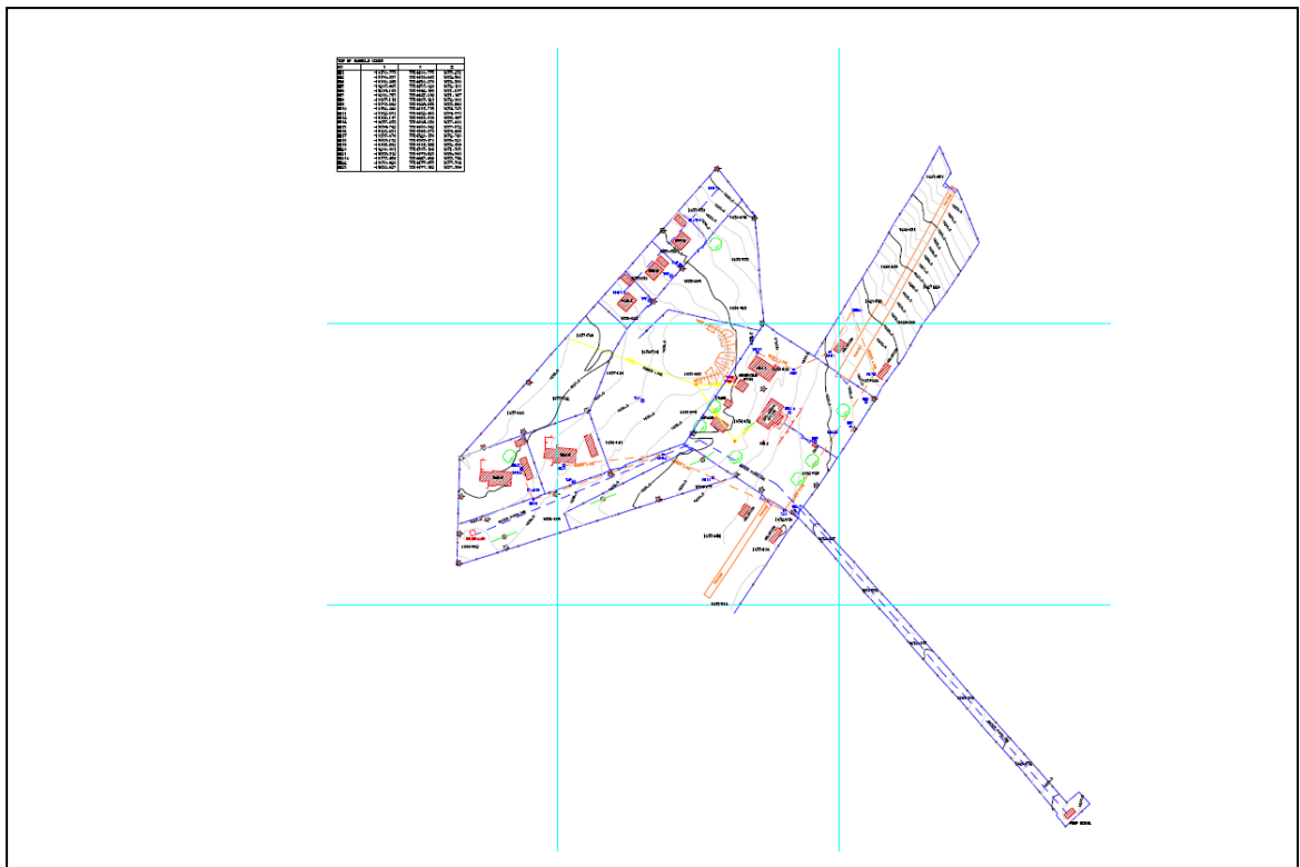
Figure 2.3: Sepapushek Port of Entry: Site Layout
