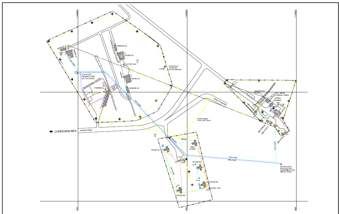
Figure 2.2: Telle Bridge Port of Entry: Site Layout
