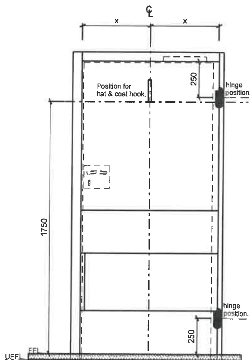
TYPICAL ELEVATION - HAT & COAT HOOK
