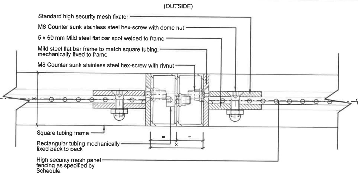
DETAIL C 'SCALE 1:2'
