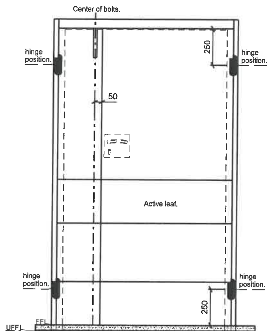
TYPICAL ELEVATION - FLUSH BOLT INSTALLATION
