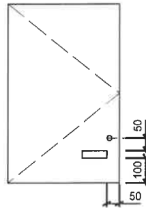
WALL CUPBOARD
