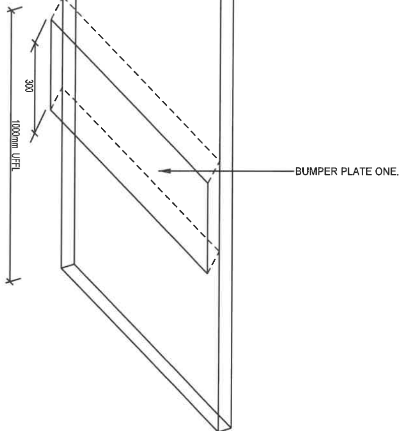
PROTECTION PLATE TYPE E: (SINGLE AND DOUBLE DOORS WITHOUT EDGE PROTECTION). ELEVATION 1:10
