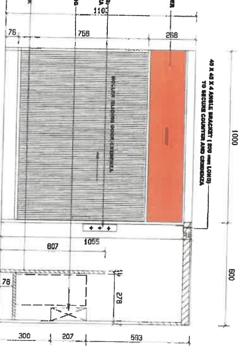
SECTIONAL ELEVATION C-C SCALE 1:20
